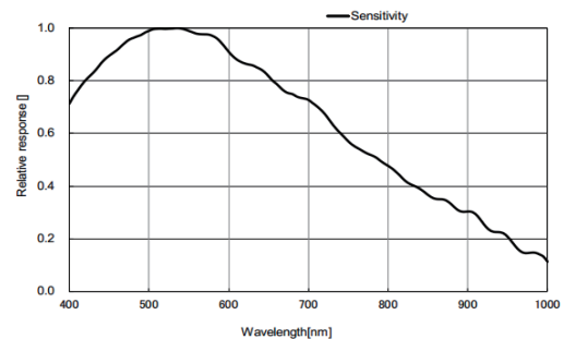
CK-U1200MI-10RS 响应曲线
