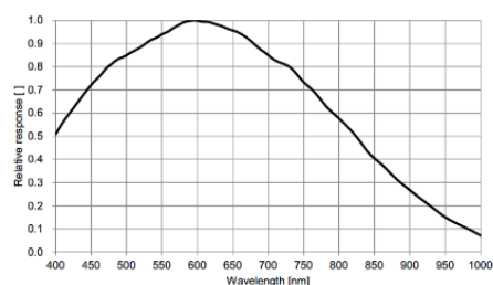
CK-H1200MU-23GS 量子效率
